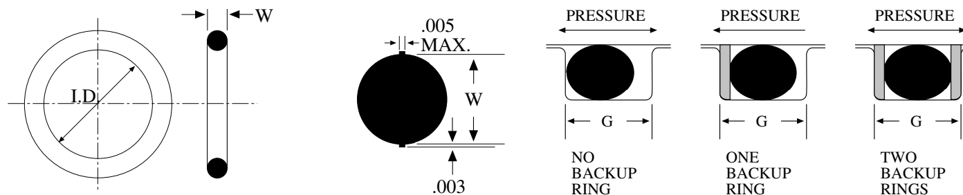
GLAND DETAIL
