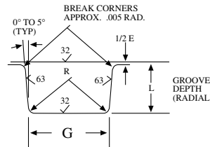
GLAND DETAIL
