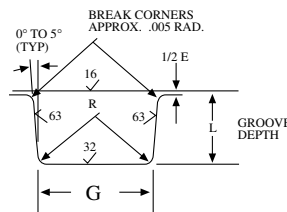
GLAND DETAIL
