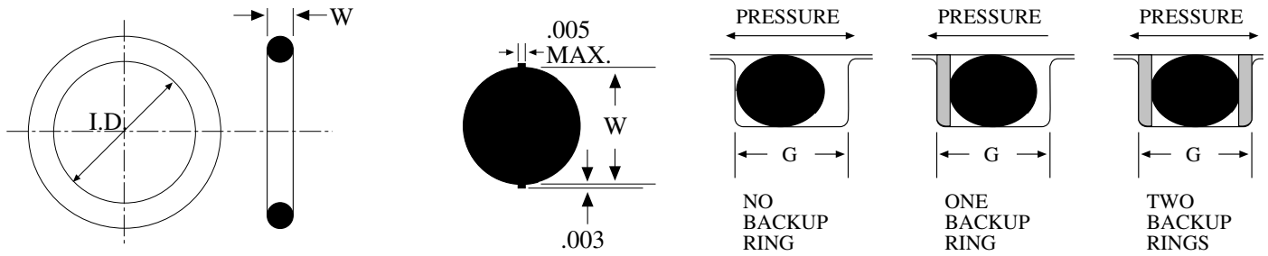
GLAND DETAIL
